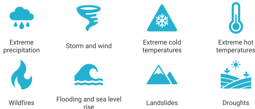
Figure 3 Types of climate hazards considered
