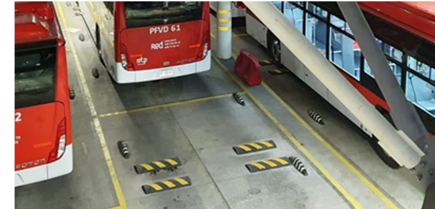
Figure 16. Stopping points on the floor of a bus depot inform the driver they have reached the desired stopping location.
